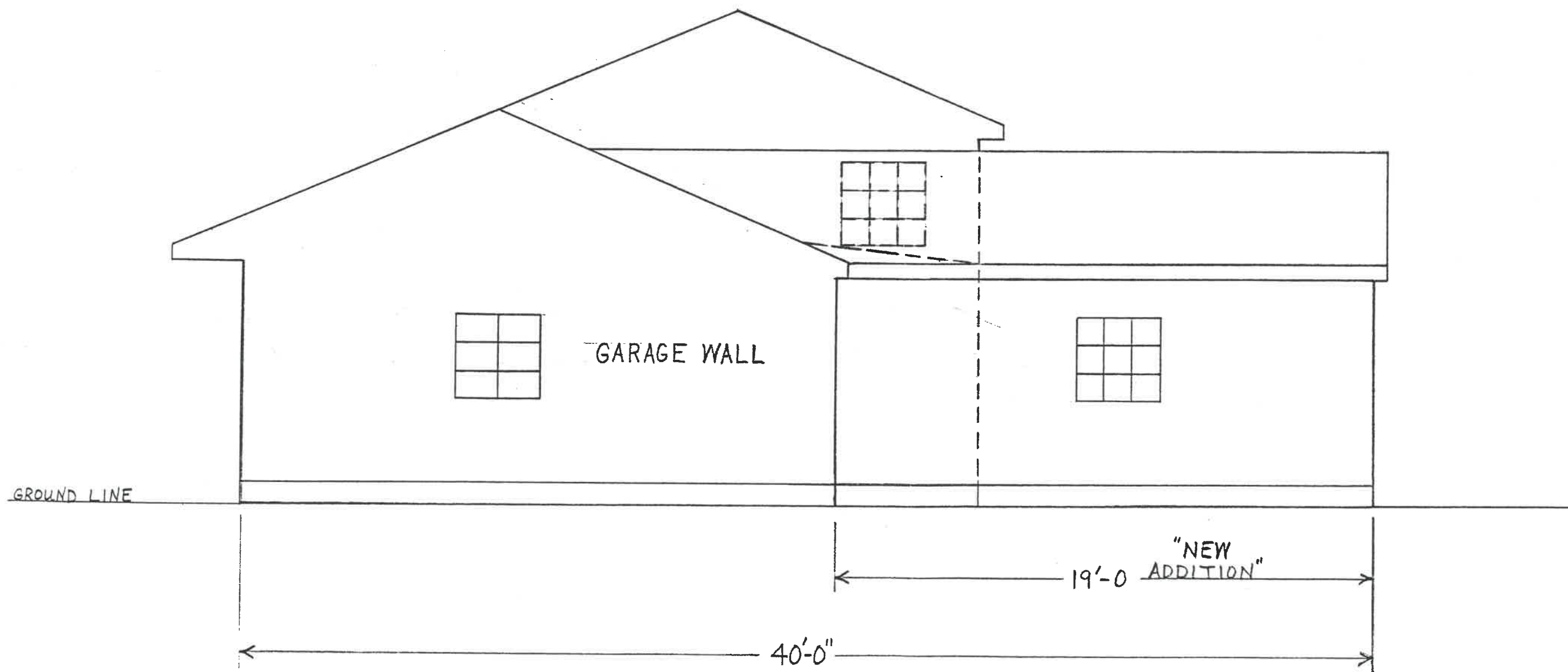
EAST ELEVATION - \frac{1}{4}'' = 1 FOOT SCALE
